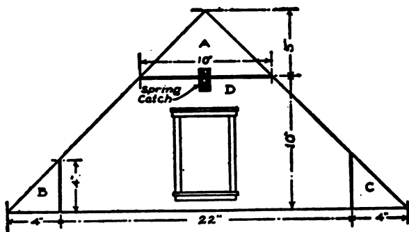
FIG. 233. — The Front Gable-End.
